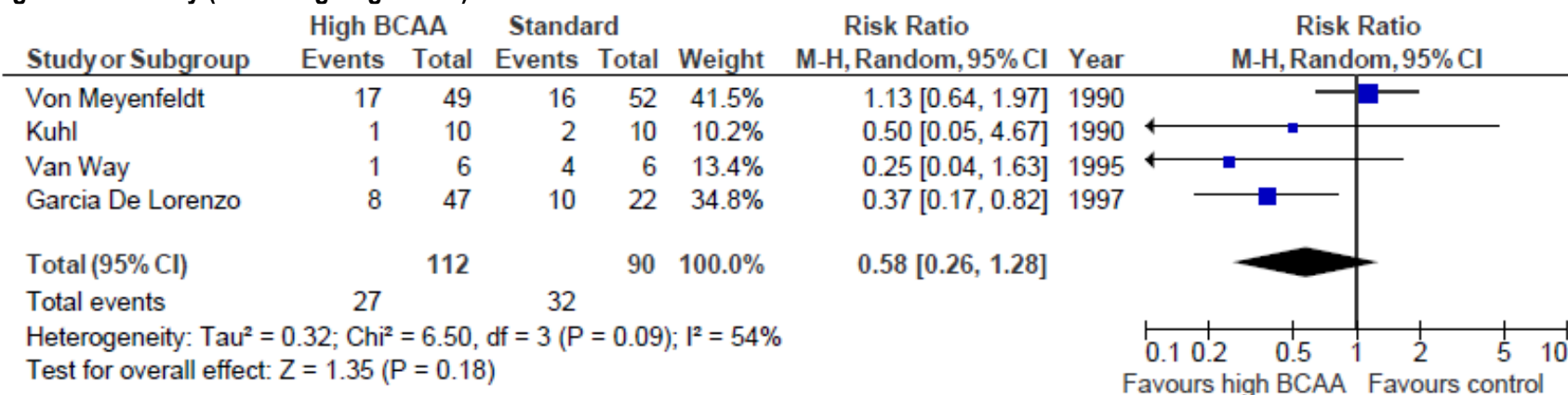
Figure 2. Mortality (excluding Ozgultekin)
